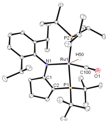
Figure 2. ORTEP drawing of the solid-state molecular structure of 6c with probability ellipsoids at 50%. Hydrogen atoms are omitted for clarity, with the exception of H50, which was found in the difference map. Selected bond lengths (Å) and angles (deg): Ru1–N1 2.1427(2), Ru1–P1 2.3576(4), Ru1–P2 2.4217(4), Ru1–C100 1.8228(2), N1–C1 1.3774(2), C1–C2 1.372(2), C2–P1 1.7703(2), C100–O1 1.169(2), N1–C1–C2 125.24(2), C1–C2–P1 113.94(1), N1–Ru1–P1 81.05(3), C100–Ru1–P1 90.21(5), N1–Ru1–P2 106.19(3), P1–Ru1–P2 169.060(2), N1–Ru1–C100 164.25(6), C100–Ru1–H50 85(1).
