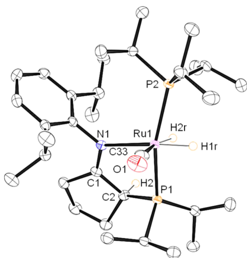
Figure 3. ORTEP drawing of the solid-state molecular structure of 7a with probability ellipsoids at 50%. All of the hydrogen atoms except \alpha -CH proton and hydrides are omitted for clarity. The \alpha -CH proton and hydrides were located in the difference map. Selected bond lengths ( \text{\AA} ) and angles ( ^\circ ): Ru1–N1 2.306(3), Ru1–P1 2.2923(2), Ru1–P2 2.3310(2), Ru1–C32 1.872(6), N1–C1 1.293(6), C1–C2 1.510(6), C2–P1 1.854(5), C32–O1 1.172(6), N1–C1–C2 122.3(4), C1–C2–P1 109.1(3), N1–Ru1–P1 80.82(9), C33–Ru1–P1 100.50(2), N1–Ru1–P2 107.77(9), P1–Ru1–P2 161.99(4), N1–Ru1–C33 101.33(2).
