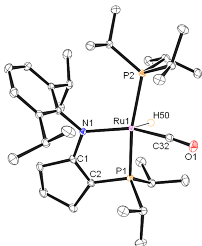
Figure 1. ORTEP drawing of the solid-state molecular structure of 6a with probability ellipsoids at 50%. Hydrogen atoms are omitted for clarity, with the exception of H50, which was found in the difference map. Selected bond lengths (Å) and angles (deg): Ru1–N1 2.1287(2), Ru1–P1 2.3273(6), Ru1–P2 2.4081(6), Ru1–C32 1.8196(2), N1–C1 1.3796(2), C1–C2 1.3643(2), C2–P1 1.7629(2), C32–O1 1.1640(2), N1–C1–C2 125.42(2), C1–C2–P1 113.52(2), N1–Ru1–P1 81.47(4), C32–Ru1–P1 88.62(5), N1–Ru1–P2 106.42(4), P1–Ru1–P2 166.600(2), N1–Ru1–C32 155.36(5), C32–Ru1–H50 84.1(7).
